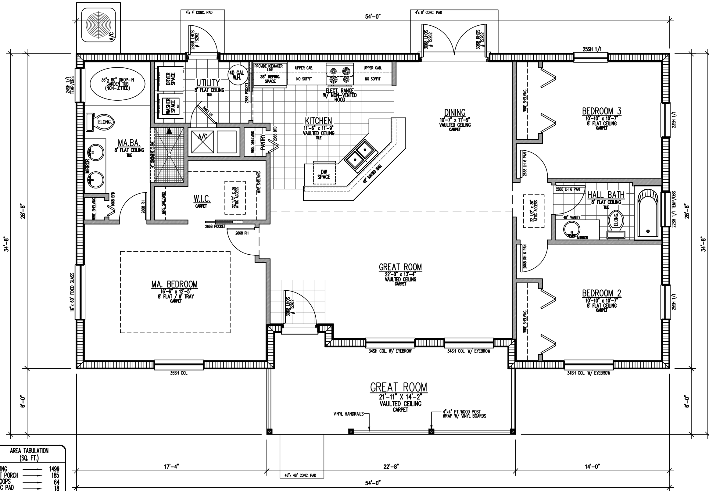
2 FLOOR PLAN 3/16"=1'-0"
