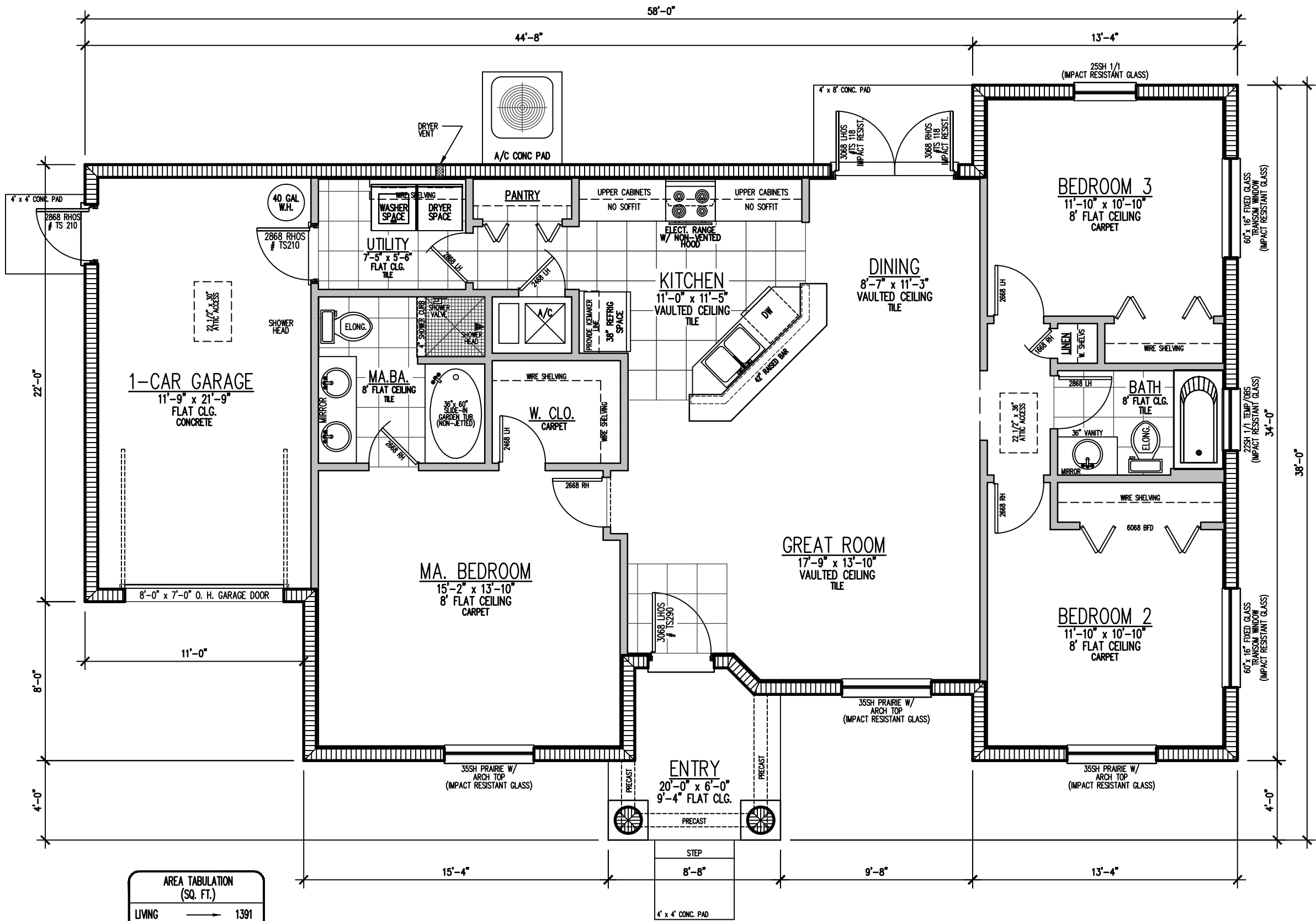
2 FLOOR PLAN 3/16"=1'-0"
