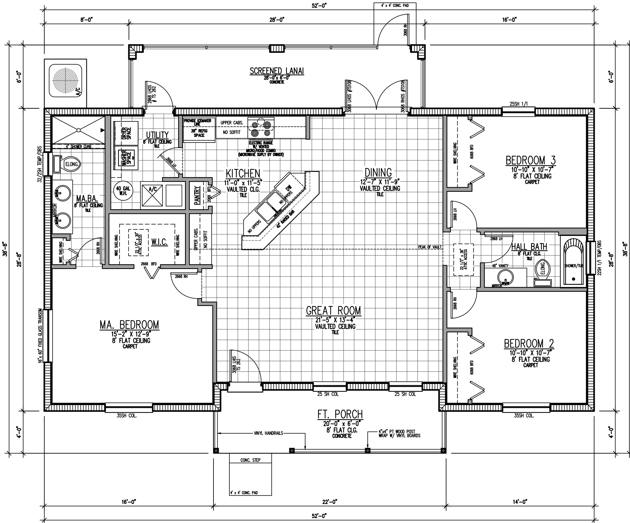
2 FLOOR PLAN 3/16"=1'-0"
