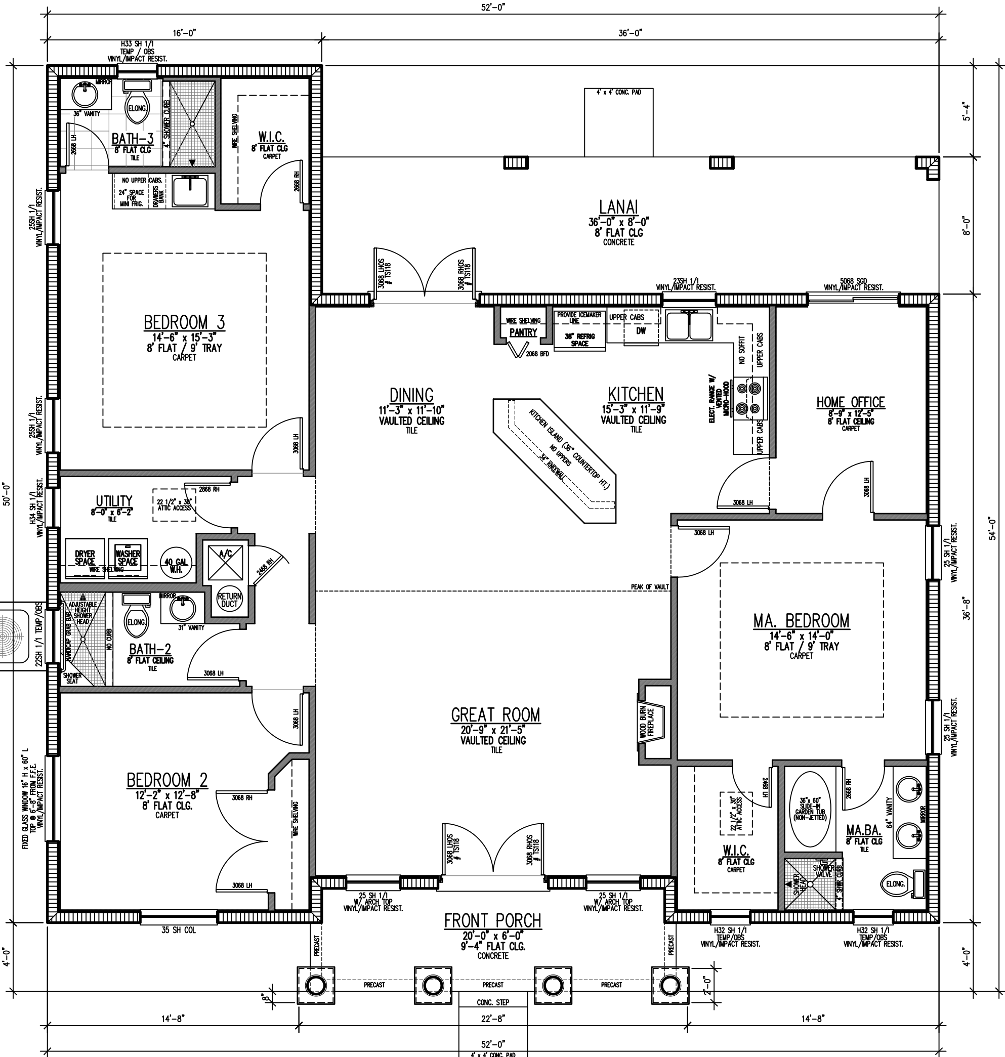
2 FLOOR PLAN 3/16"=1'-0"
