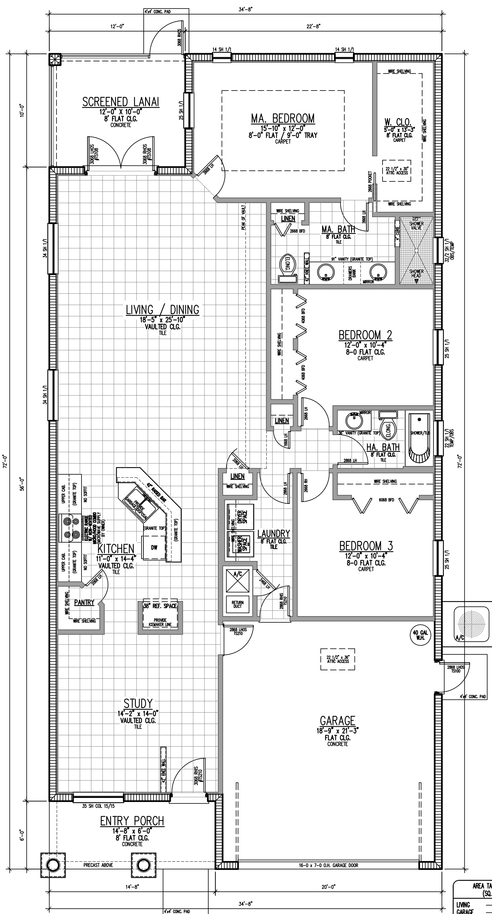
1 FLOOR PLAN 1/4" = 1'-0"
