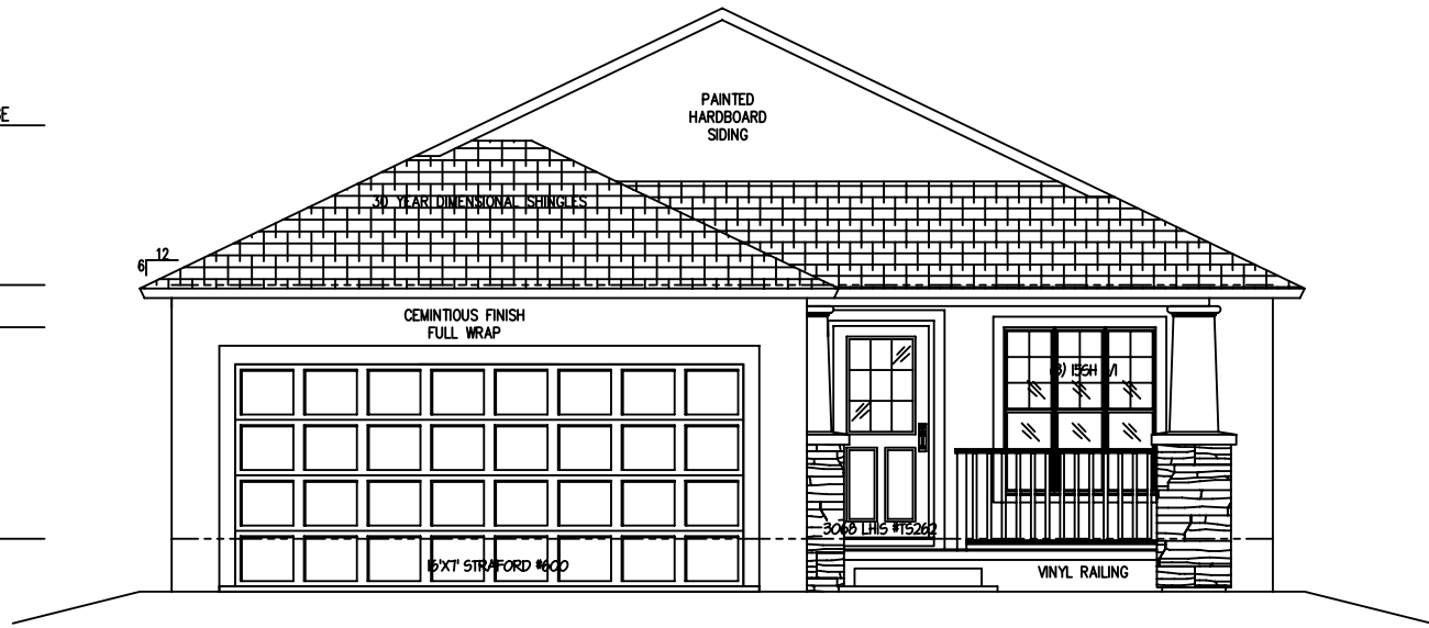
1 FRONT ELEVATION 1/4"=1'-0"
