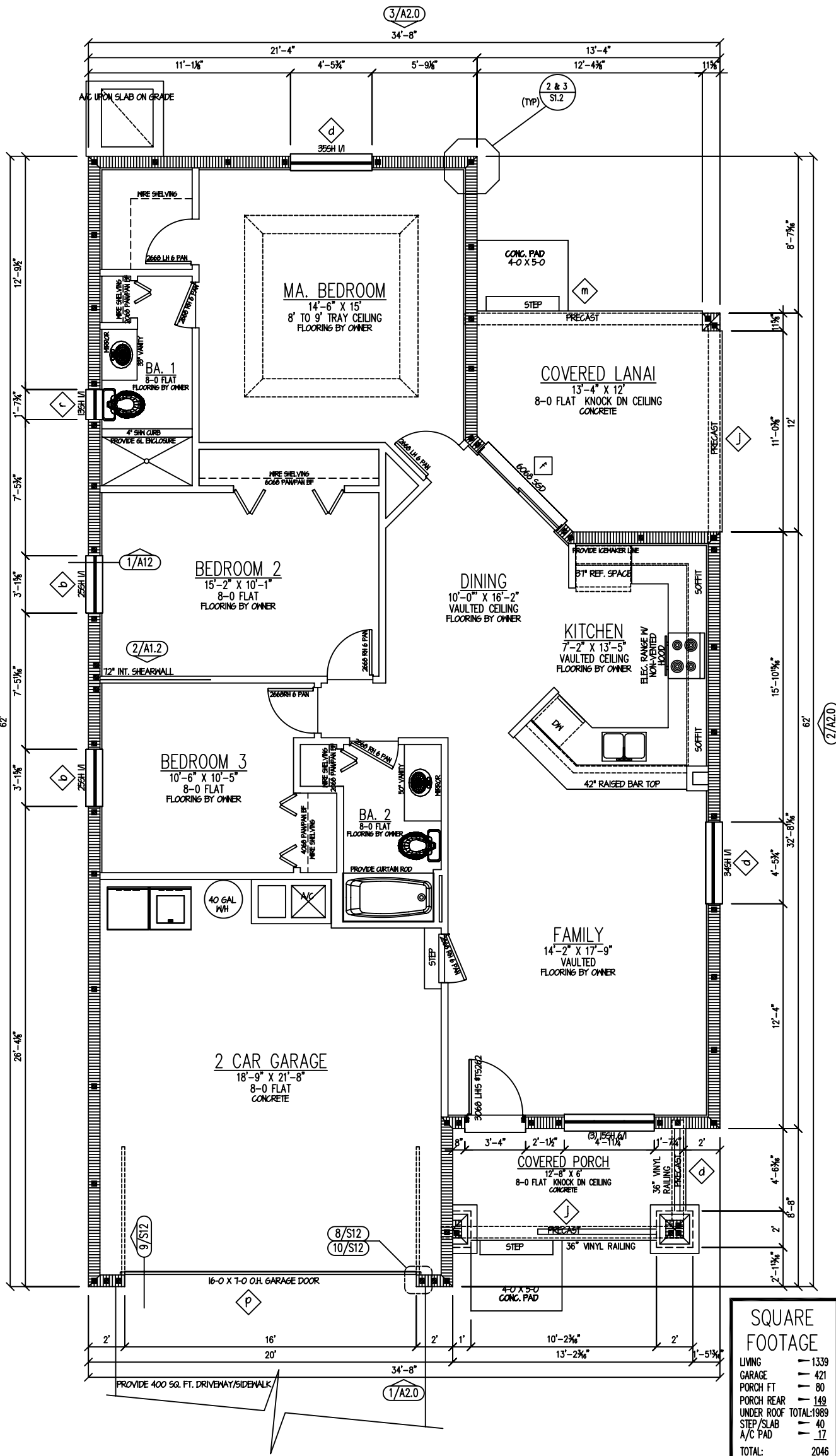
2 FLOOR PLAN 1/4"=1'-0"
