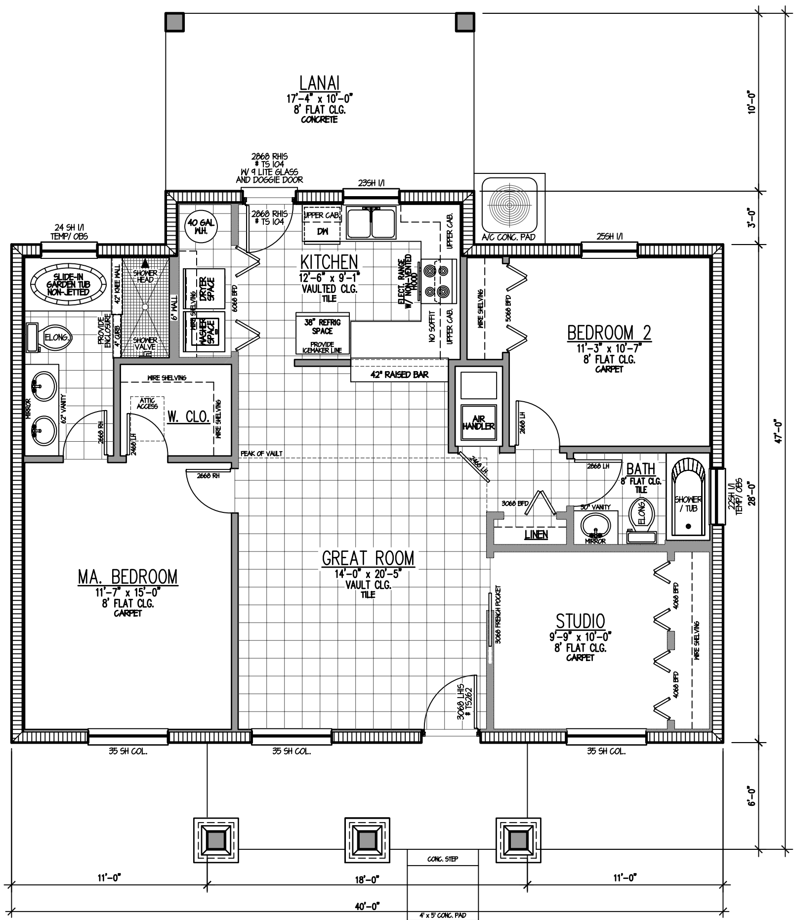
1 FLOOR PLAN 3/16" = 1'-0"
