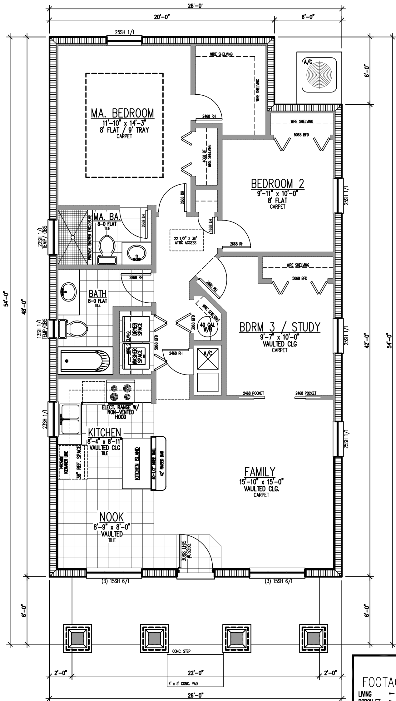
2 FLOOR PLAN 3/16" = 1'-0" HA8908 DAVIDSON 05/13/10
