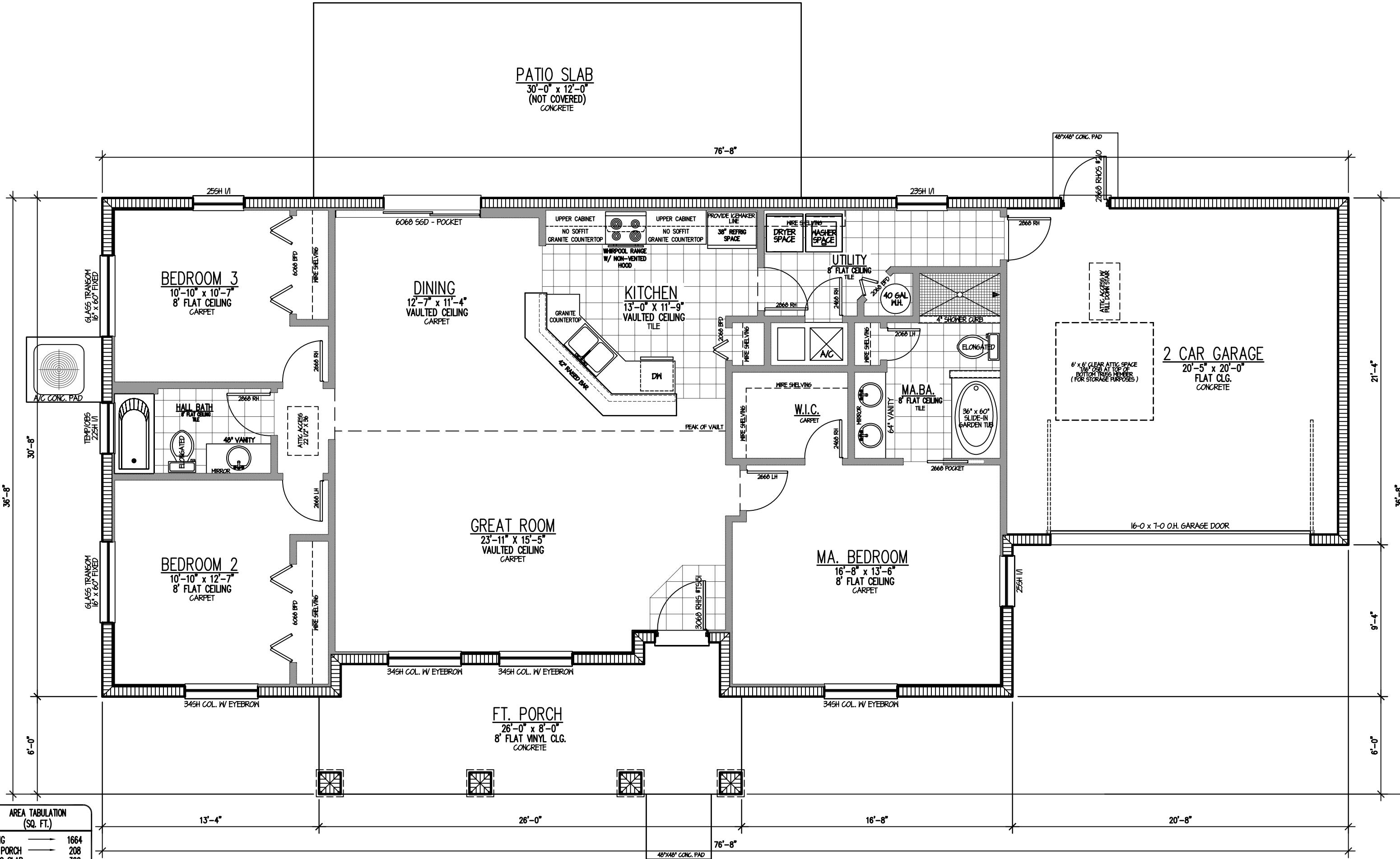
2 FLOOR PLAN 3/16"=1'-0"
