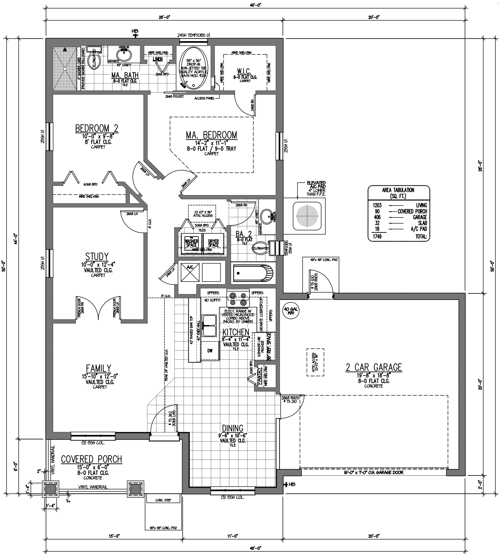
2 FLOOR PLAN 3/16" = 1'-0"
