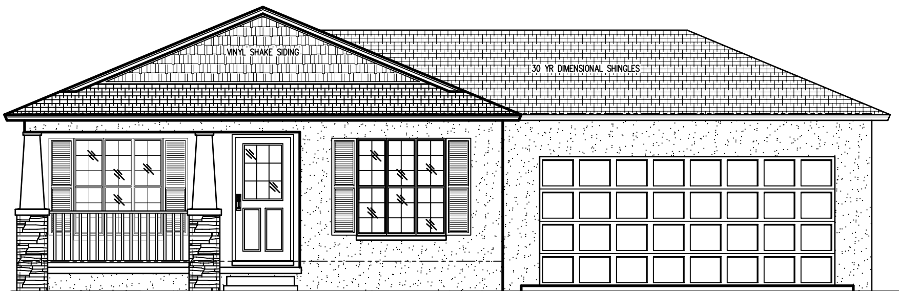
1 FRONT ELEVATION 3/16" = 1'-0"
