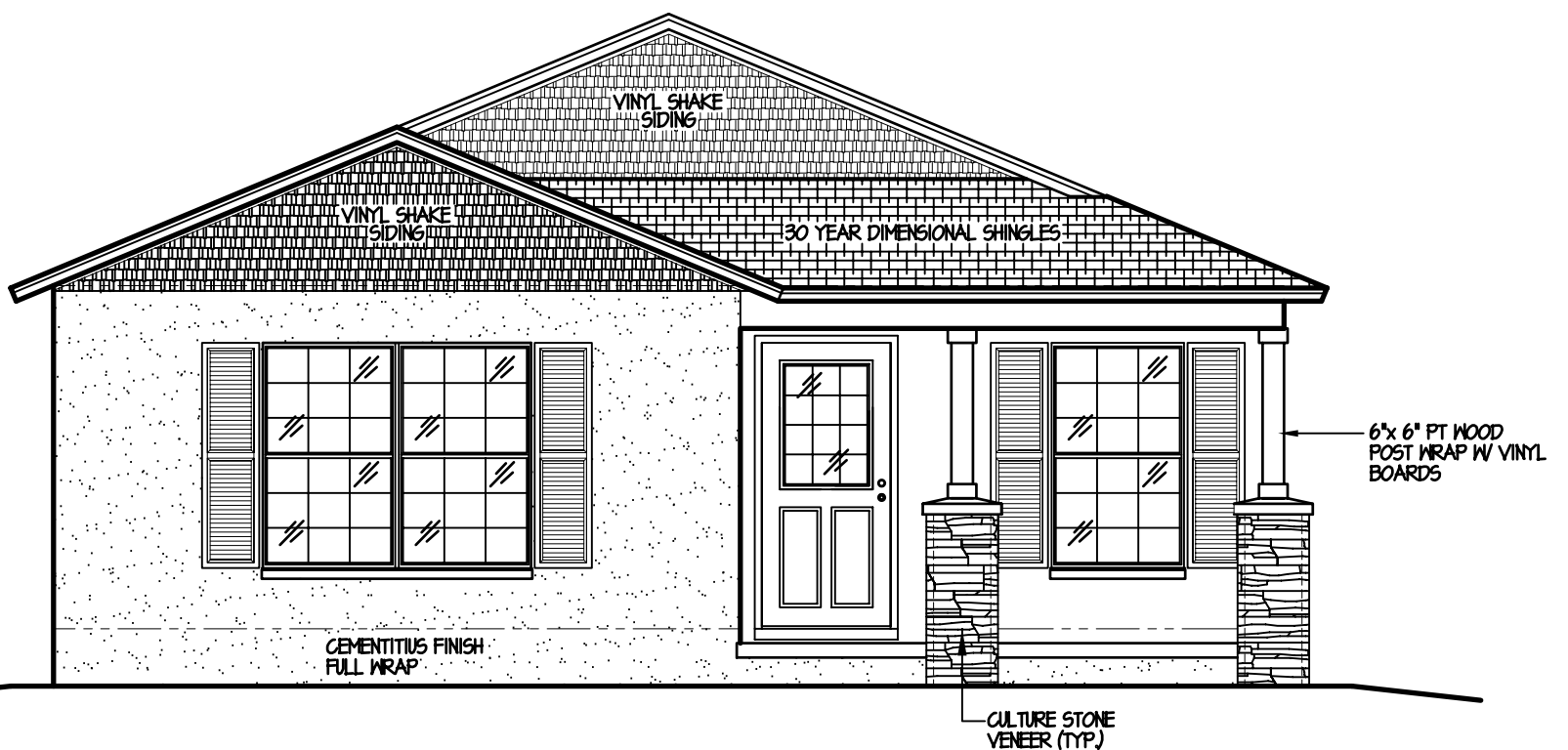
1 FRONT ELEVATION 3/16"=1'-0"
