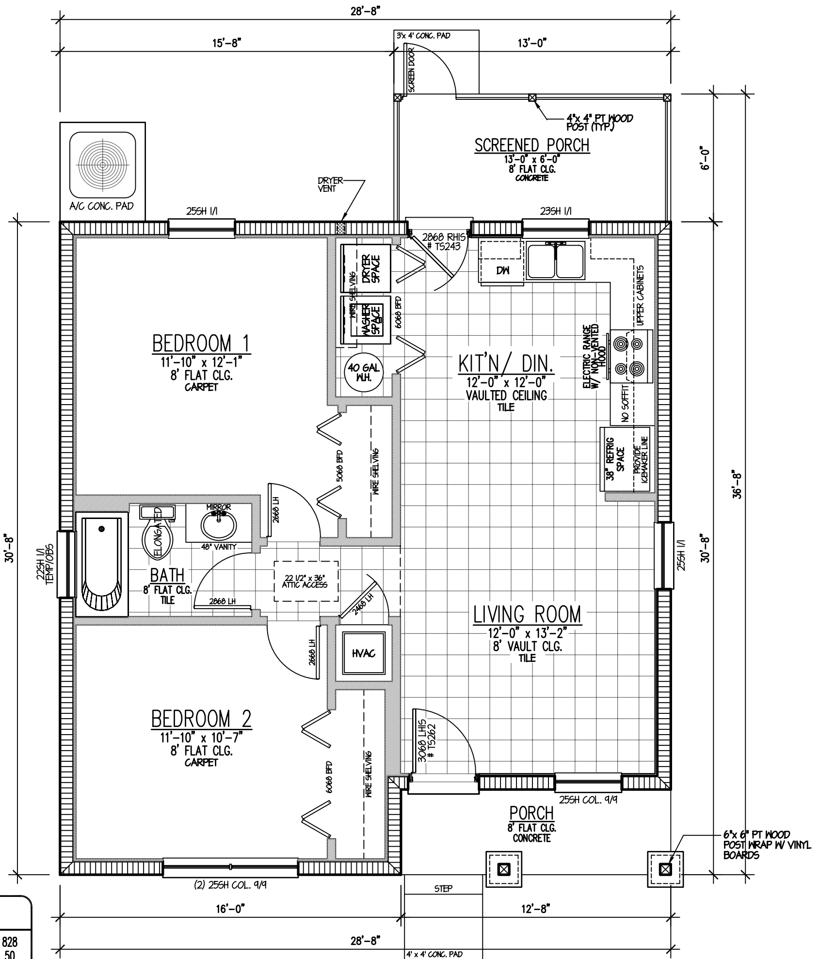
2 FLOOR PLAN 3/16"=1'-0"
