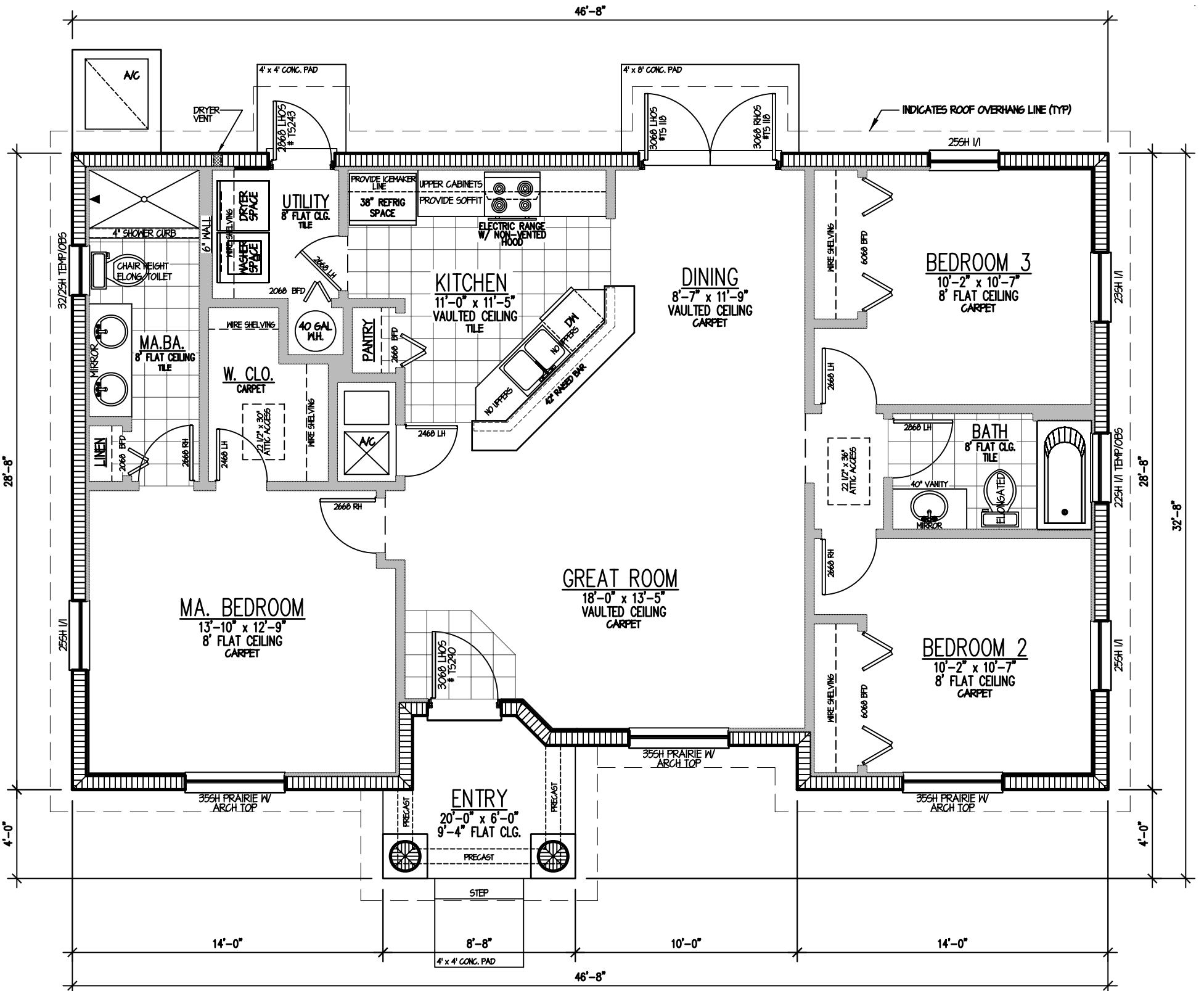
2 FLOOR PLAN 3/16"=1'-0"
