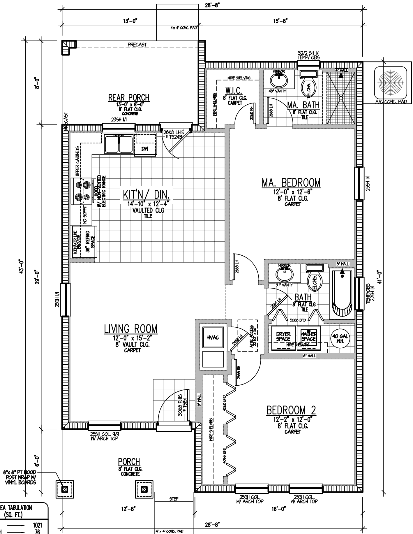
2 FLOOR PLAN 3/16"=1'-0" HA9003 HANCOCK 10/27/10
