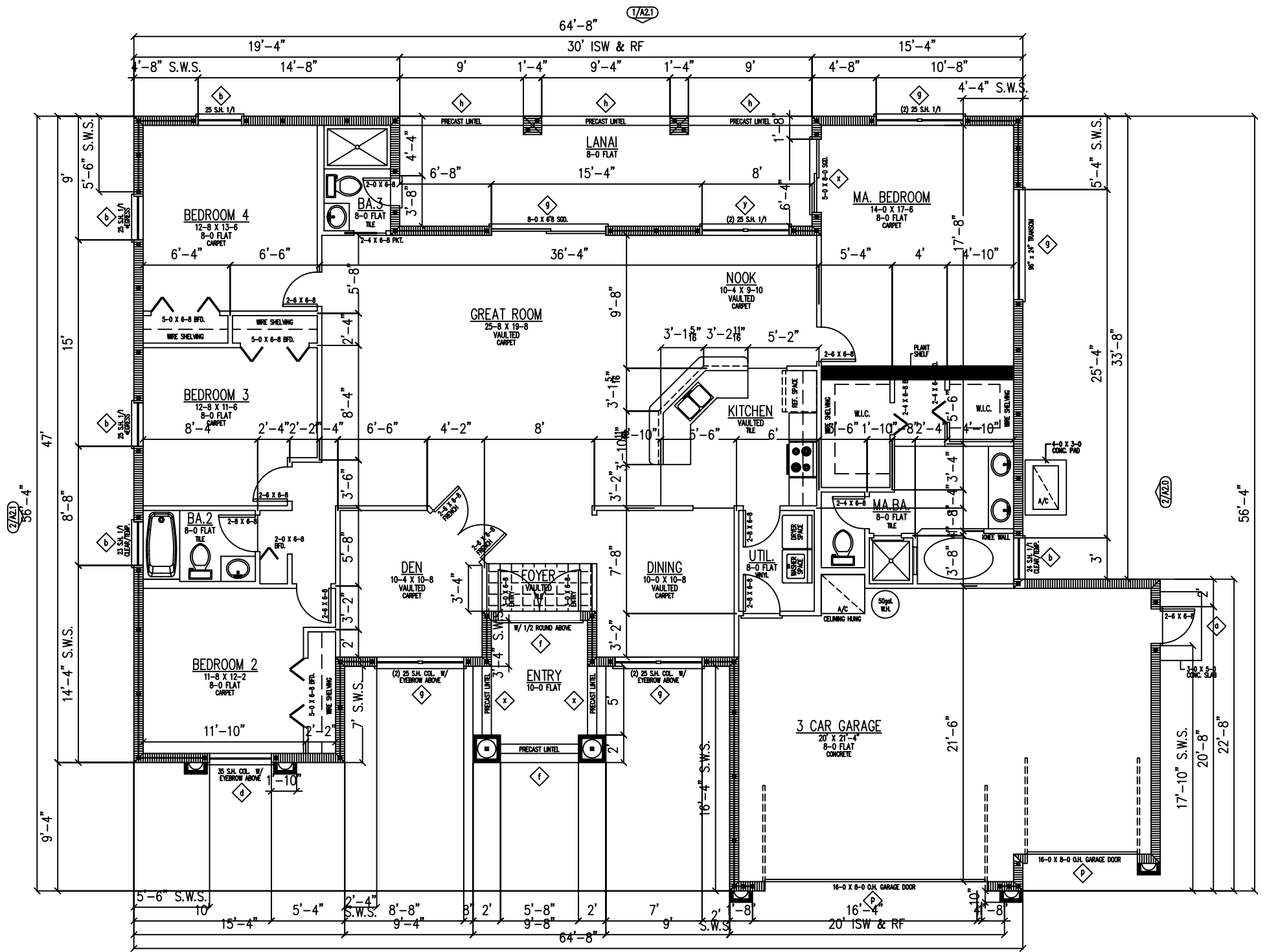
1 FLOOR PLAN 1/4" = 1'-0"
