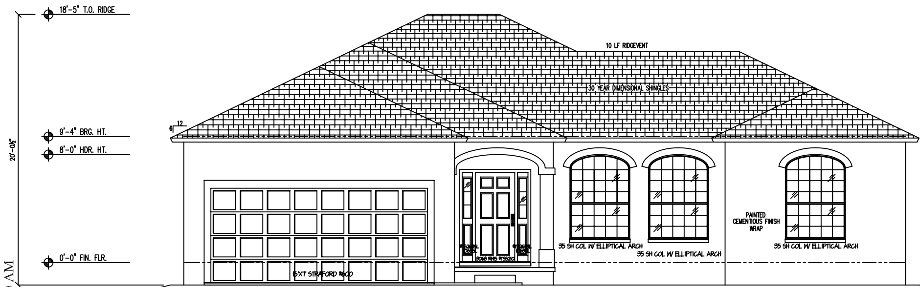
1 FRONT ELEVATION 1/4" = 1'-0"
