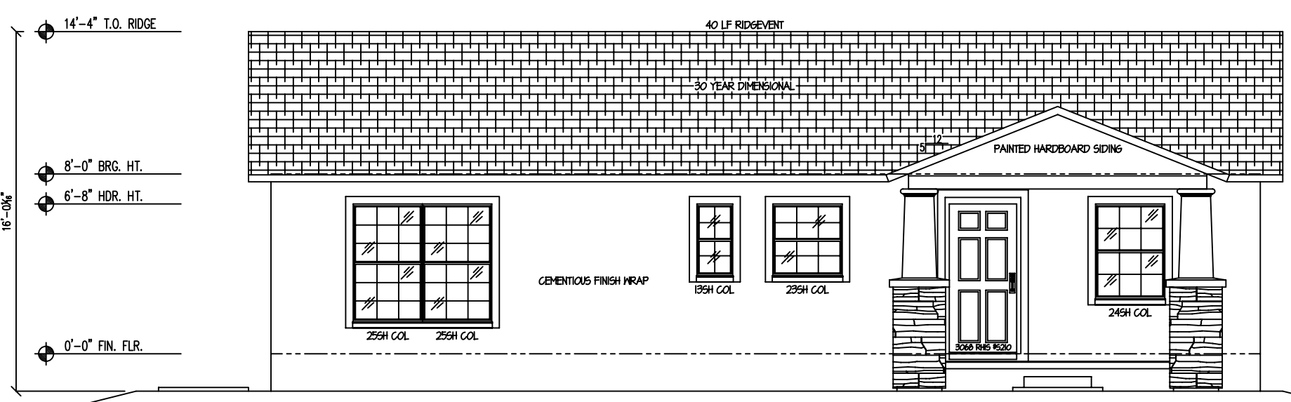
1 FRONT ELEVATION 1/4" = 1'-0"
