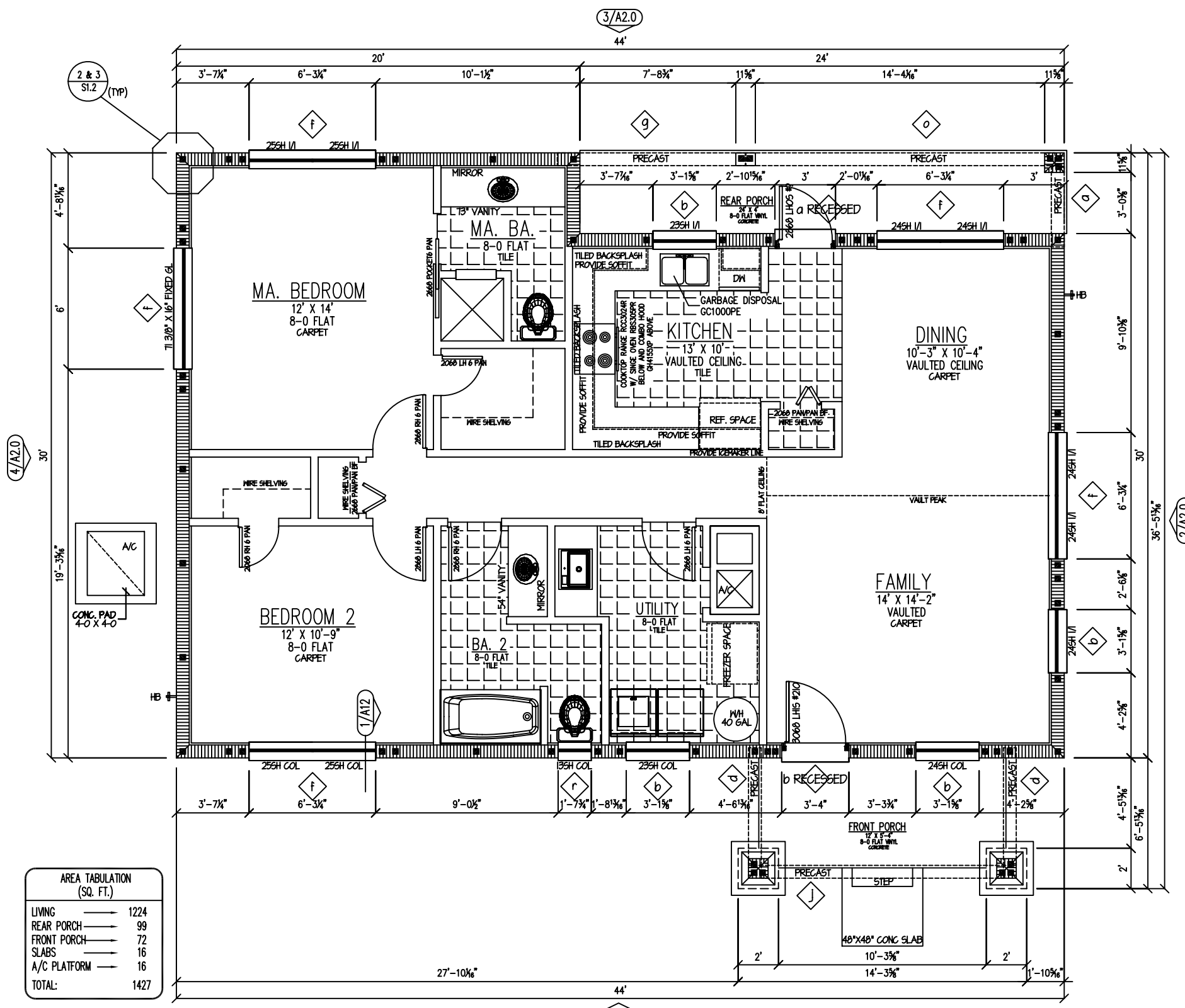
2 FLOOR PLAN 1/4" = 1'-0" ALL EXTERIOR WALLS BETWEEN DOOR & WINDOW JAMBS ARE SHEAR RESISTING COMPONENTS, EXCEPT WHERE ELECTRICAL, PLUMBING & MECHANICAL COMPONENTS ARE LOCATED
