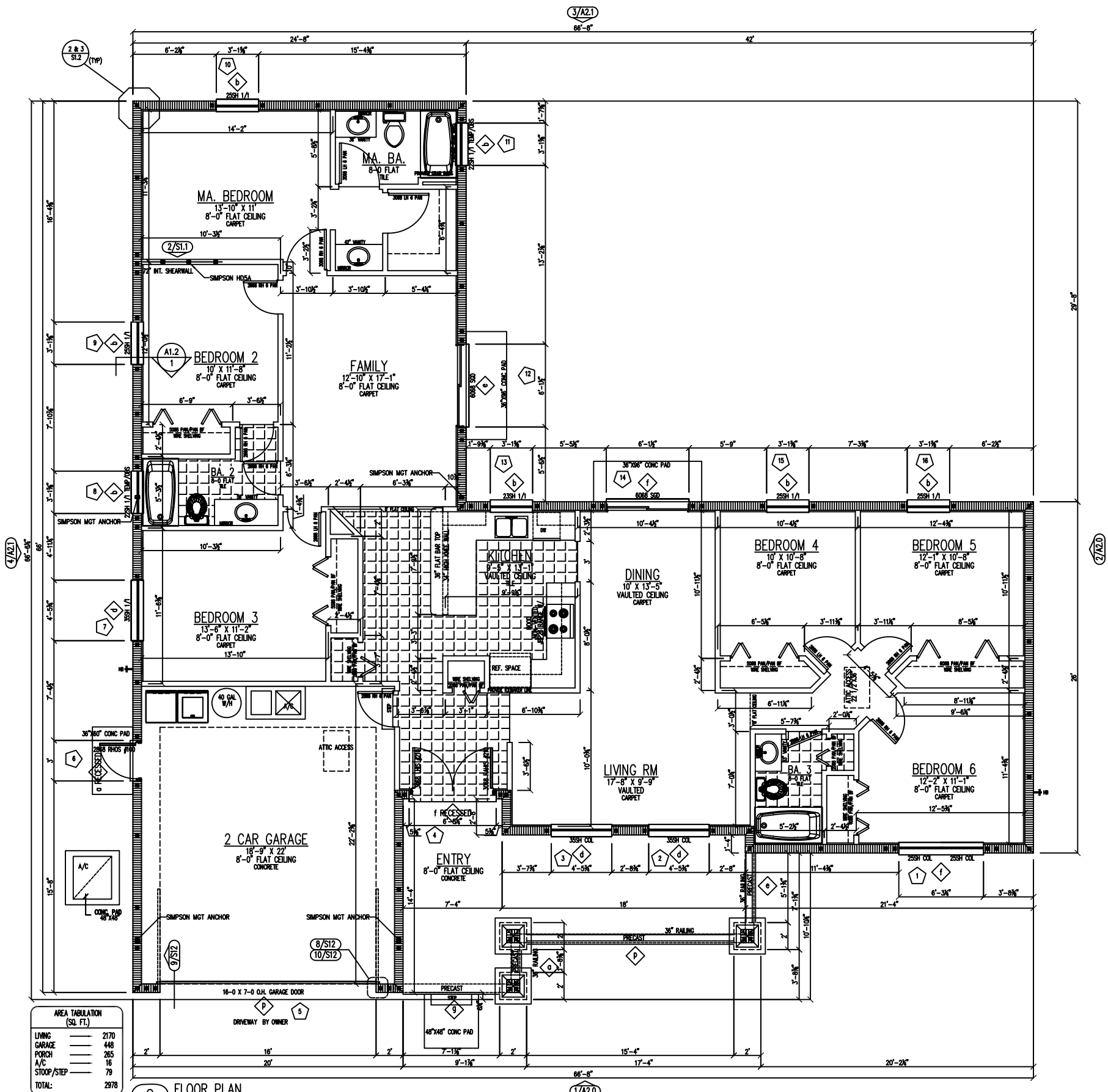
2 FLOOR PLAN 1/4" = 1'-0"
