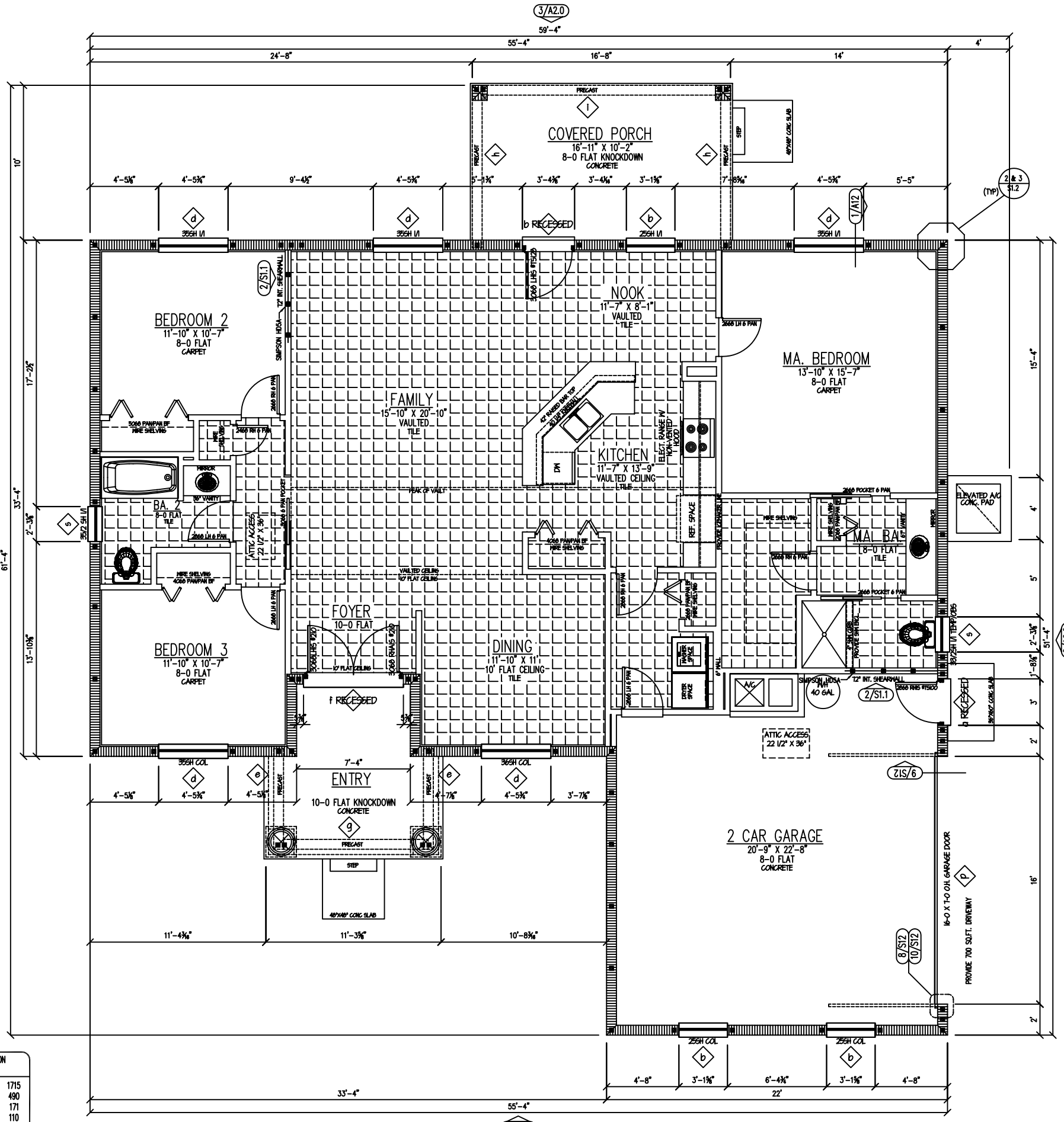
2 FLOOR PLAN 1/4" = 1'-0"
