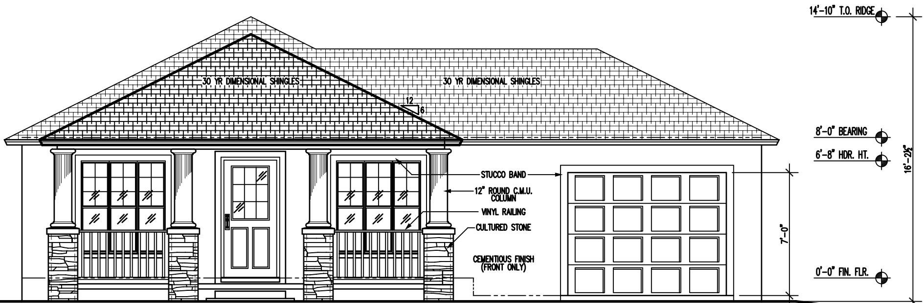
1 FRONT ELEVATION 3/16" = 1'-0"
