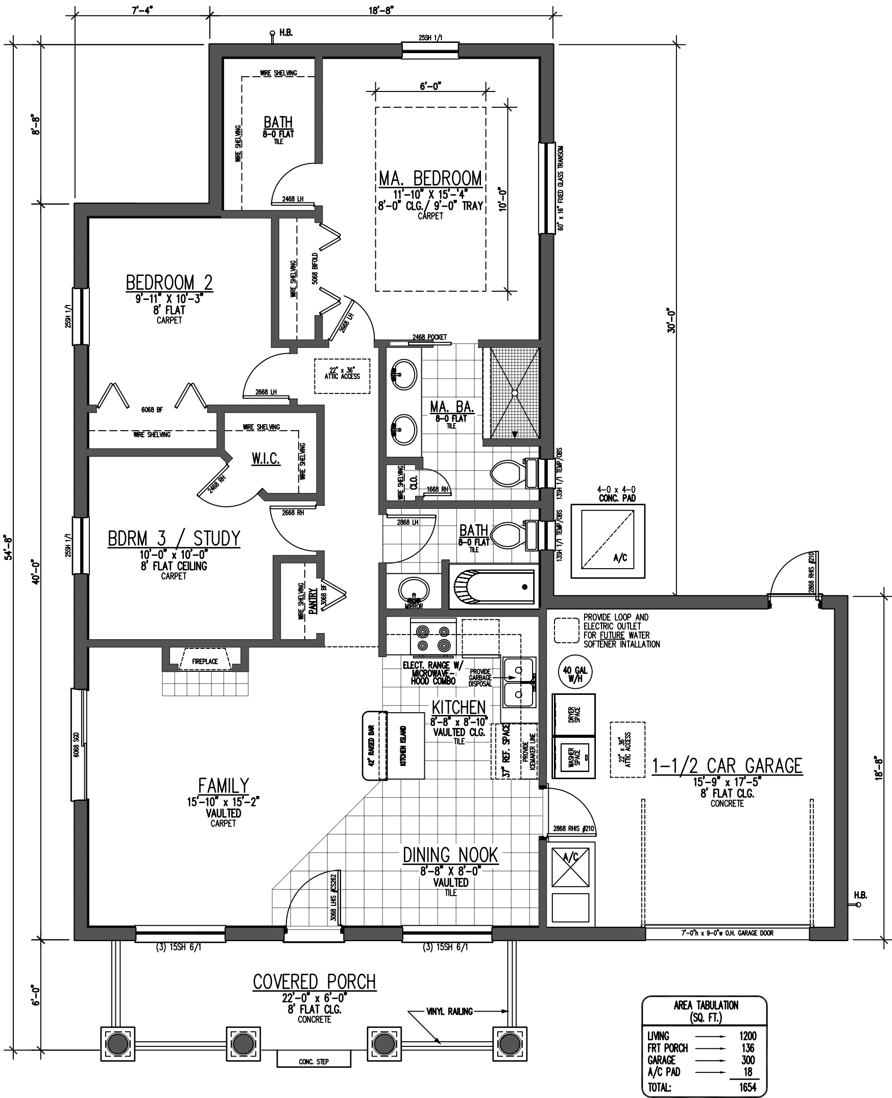
2 FLOOR PLAN 3/16" = 1'-0"
